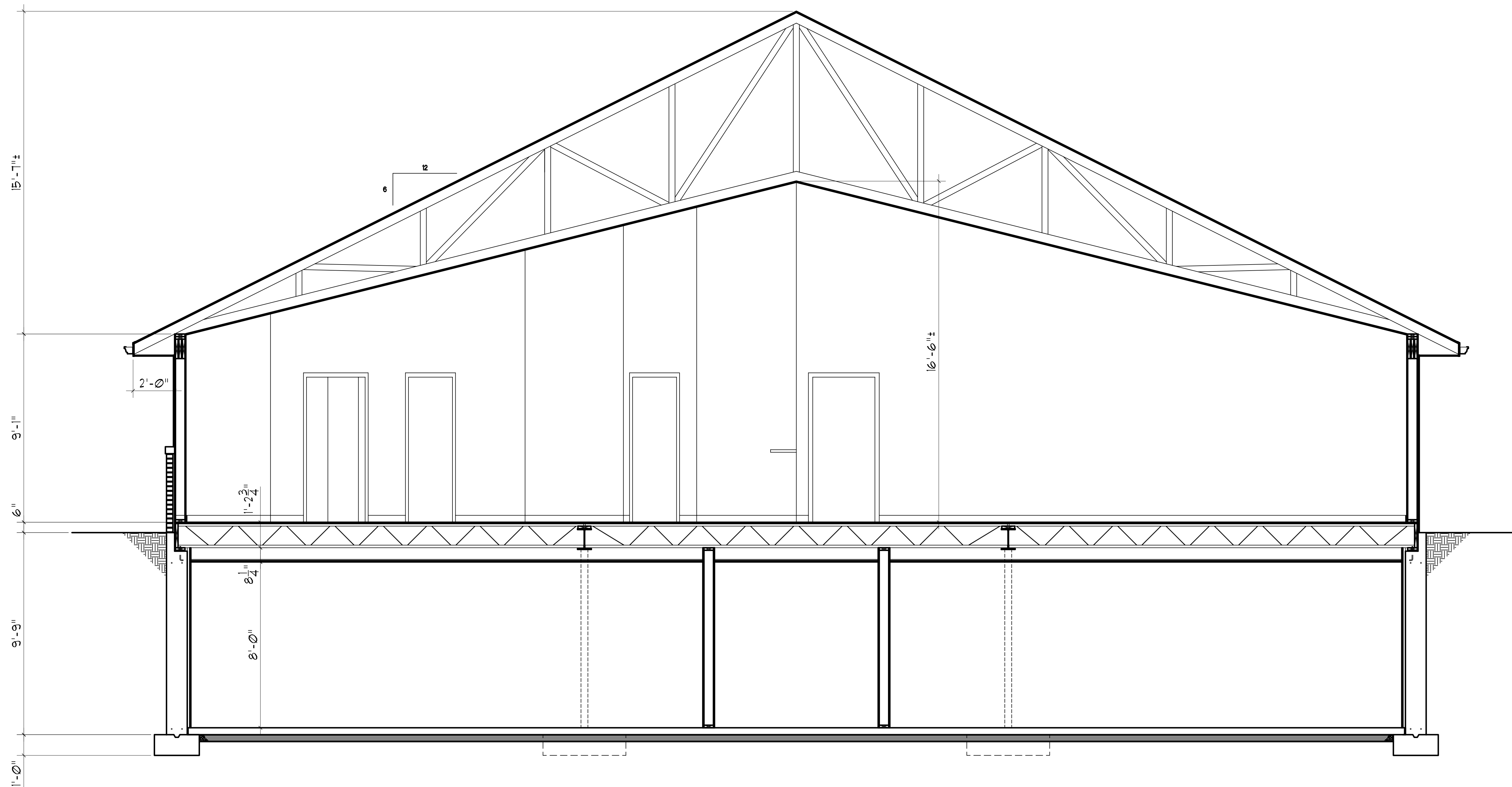
TYPICAL CROSS SECTION (FELLOWSHIP HALL and TEMPORARY SANCTUARY) SCALE: 3/4" = 1'-0"
